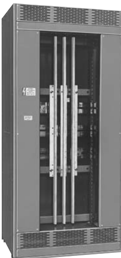
QMB Distribution Section with Neutral
